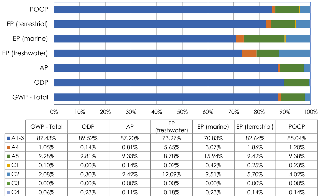
Figure 1 - shows the relative contribution of each life cycle stage to different environmental indicators for the carbon steel reinforcing bars manufactured by the DRI and secondary production route (scrap)
